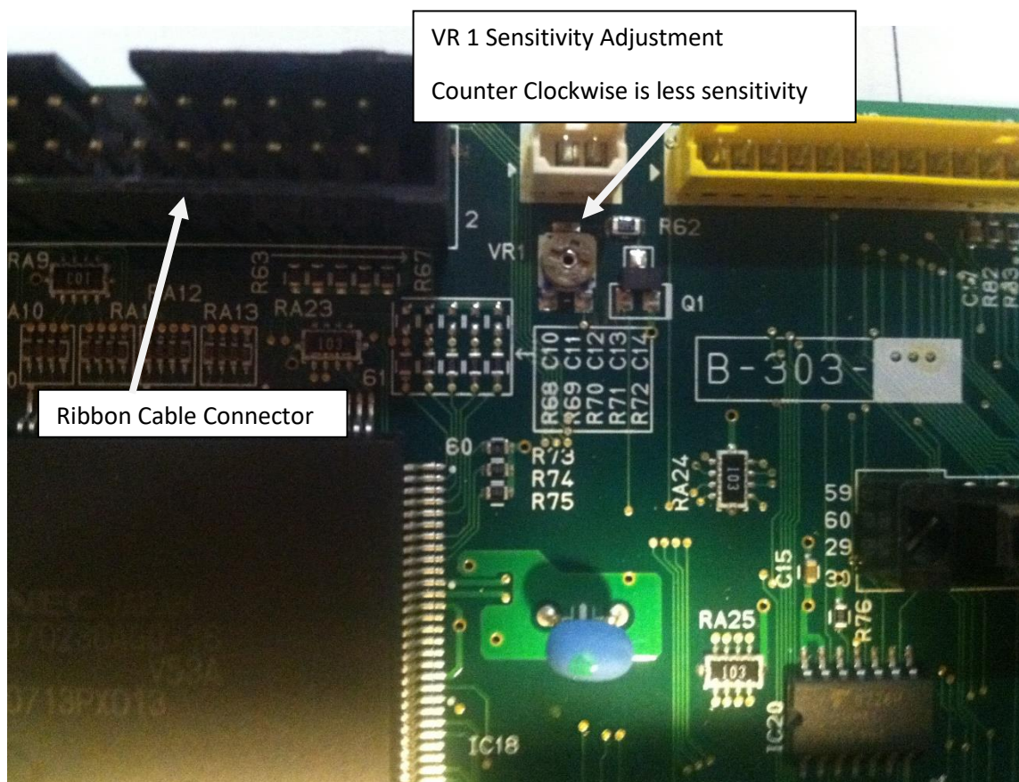
CPU Board
